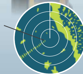
Typical radar display showing a line of dots emitted from SART
