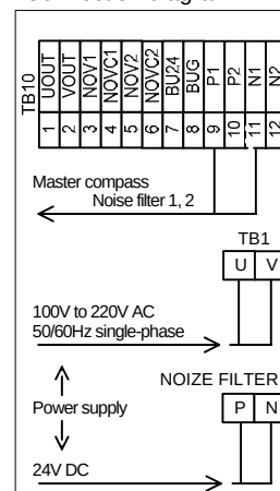
Connection diagram
